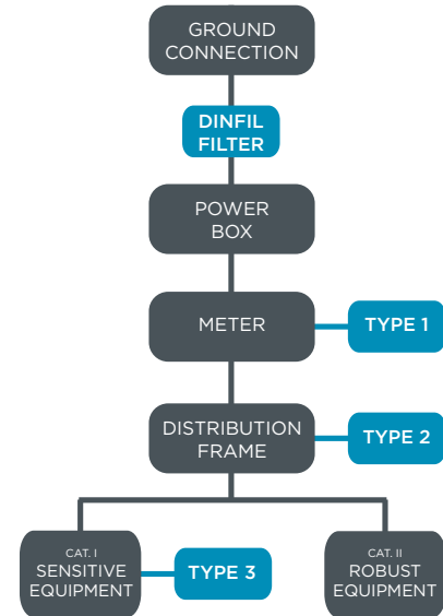
Figure 4. Electrical installation diagram.
