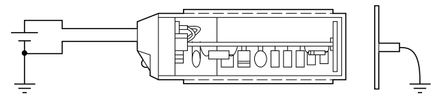
Capacitive Proximity Sensor Operation
